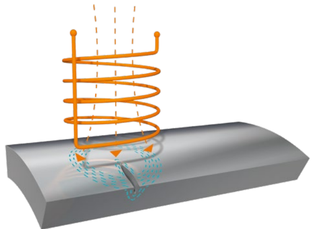
Fig. 1:Eddy Current Testing principle
