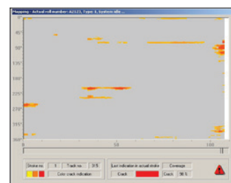
Figure 3: Mapping of scanned cylinder lining
