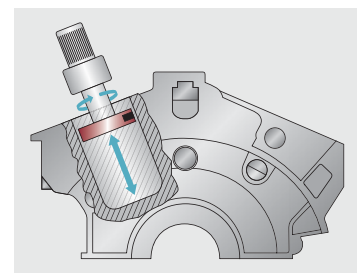
Figure 2: Testing principle
